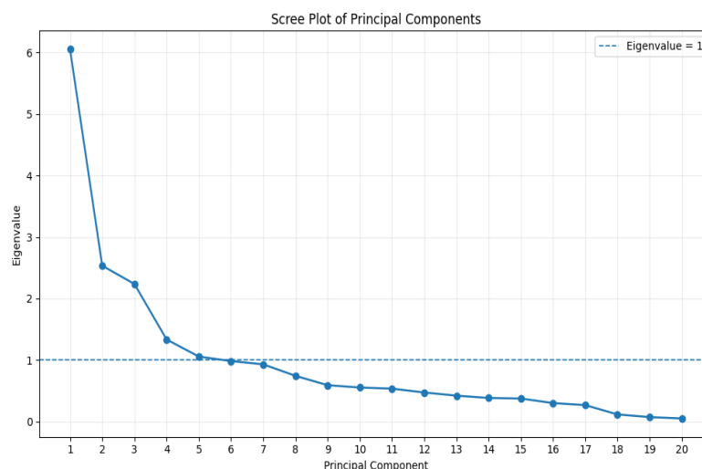
Figure 2. Scree Plot of Principal Components
