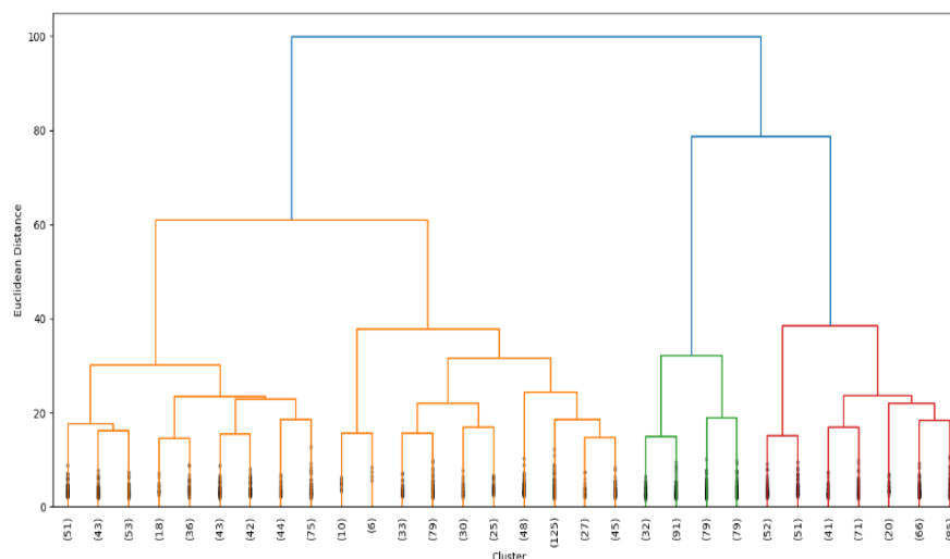
Figure 3. Hierarchical Cluster Dendrogram
