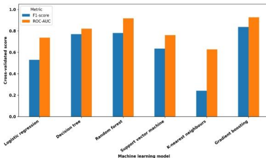
Figure 3. Cross-validated performance of the evaluated machine-learning models
