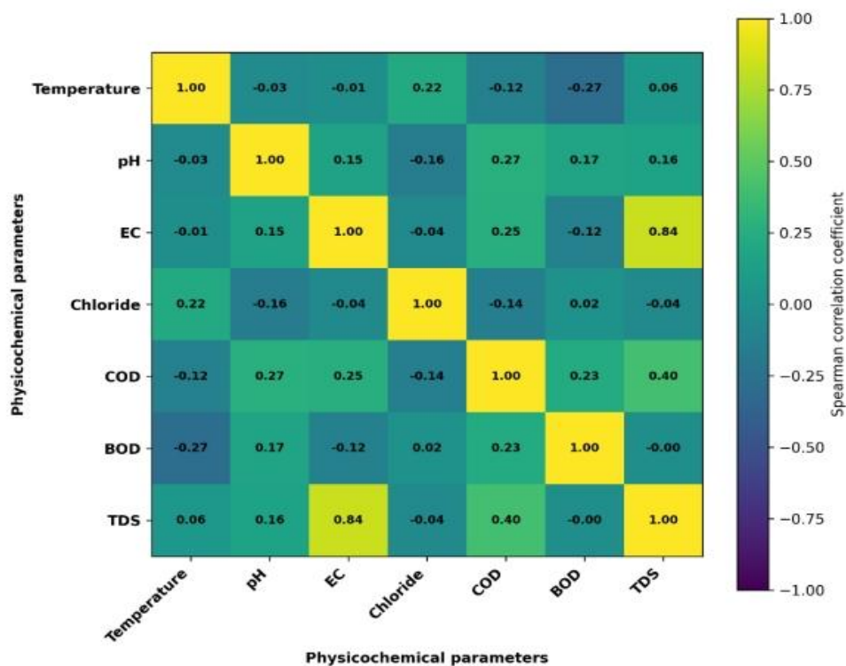
Figure 2. Spearman correlation heatmap of physicochemical water-quality parameters
